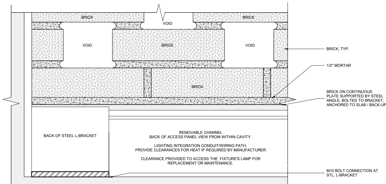
DETAIL - LIGHTING FIXTURE ACCESS - REMOVABLE CHANNEL - CAVITY VIEW BEHIND VENEER BRICK SCREEN AT BASE SUPPORT - SCALE 1:5
