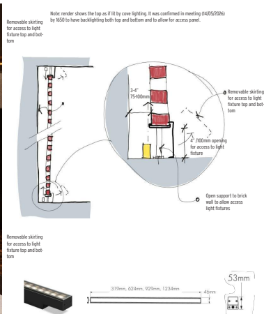
SAMPLE RENDER AND SAMPLE SKETCH OF 'HIT-AND-MISS' - PARTITION AND CONCEPT FOR BASE DETAIL - NTS
