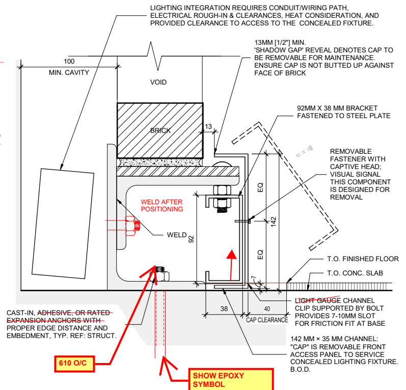
SAMPLE SKETCH : MARKUP DETAIL - COORDINATION WITH LIGHTING DESIGNER - SCALE 1:5
